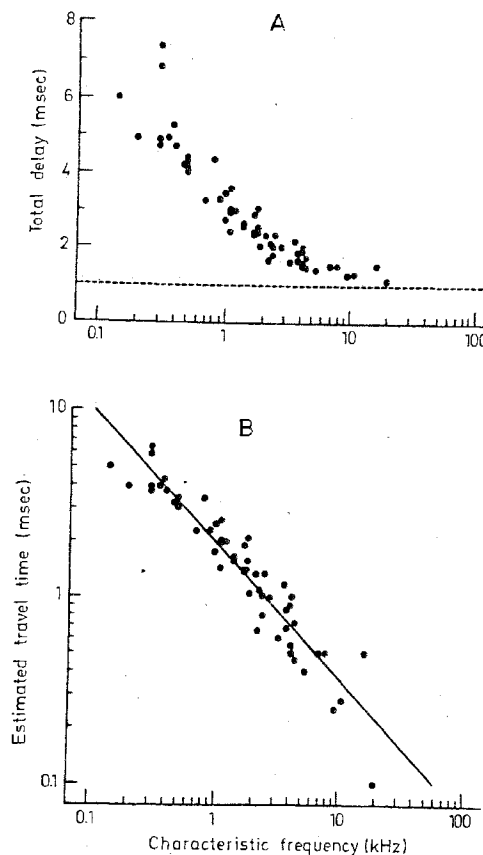
Fig. 21. A: Delay times of synchronized spike responses. 58 cochlear fibres in squirrel monkey. Delays computed from slope of phase versus frequency curves (as in Fig. 20) for each fibre, and plotted against CF of fibre. Values corrected for acoustic delay in sound system, and, therefore, represent travel time in cochlea plus synaptic and neural conduction delays. B: Cochlear travel times calculated from data of A, after subtracting 1 msec average neural delay estimated from asymptote of A (interrupted line), and plotted against each fibre's CF. (From ANDERSON et al. , 1971)
