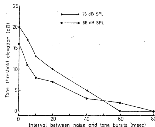
Fig. 42. "Forward masking" of unit in CN of cat. Elevation in threshold of a 10 msec test tone at CF by 40 msec broadband noise bursts at 66 or 76 dB SPL preceding the test tone by the interval indicated on the abscissa. (From WATENABE and SIMADA, 1971)
