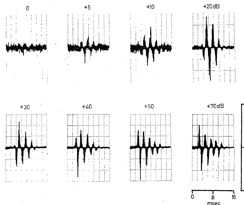
Fig. 6. Compound PST histograms of responses to click stimuli as a function of click level: Cat cochlear nerve. CF of fibre: 0.47 kHz. Click level expressed in dB relative to the "threshold" response level. Figure compiled from histograms of responses to rarefaction clicks and to condensation clicks (upper and lower halves of each compound histogram, respectively). Clicks: 100 \mu sec duration, 10/sec. Ordinate scales: linear number of spikes: 64 for 0–10 dB plots; 128 for 20 dB; 256 for 30–70 dB. (Data from KIANG et al. , 1965a)
